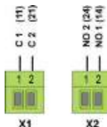
Pluggable 2-pole terminal [X1] und [X2]
