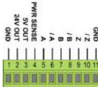
Pluggable 11-position terminal [X21], [X22]
