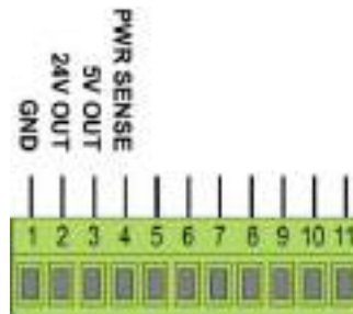
Terminals for encoder supply (24V or 5V) with optional voltage monitoring
