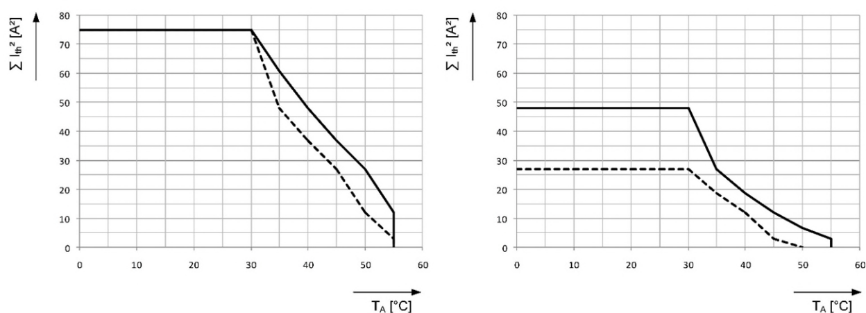
Fig. 17: Total current limit depending on the ambient temperature
