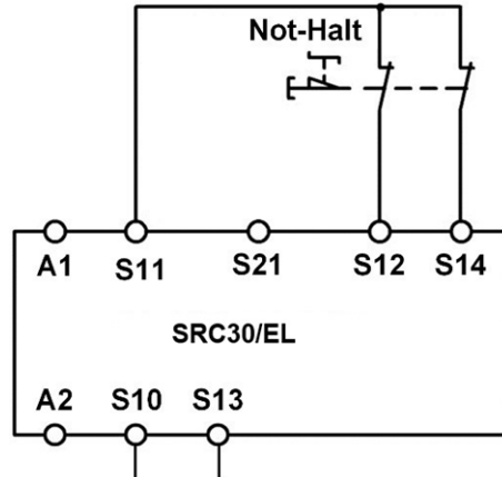
Fig. 6: Dual channel emergency stop with ground fault monitoring. (category 3, up to PL d / SIL 2)
