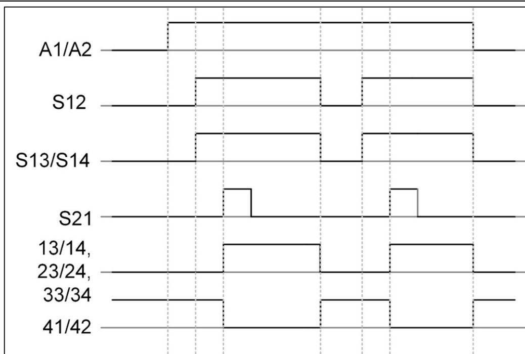
Fig. 2 State diagram
